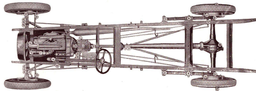
Ford Model A-A Chassis 131½" (334 cm)
